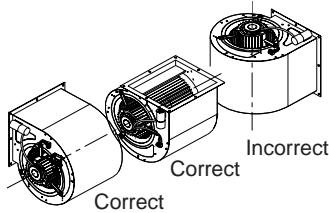
Fig.2 Standard fan mounting orientation
