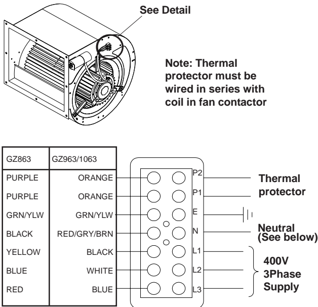
Fig.8 400V 3 Ph 50Hz SAM/REX48-3,59-3 and 510-3
